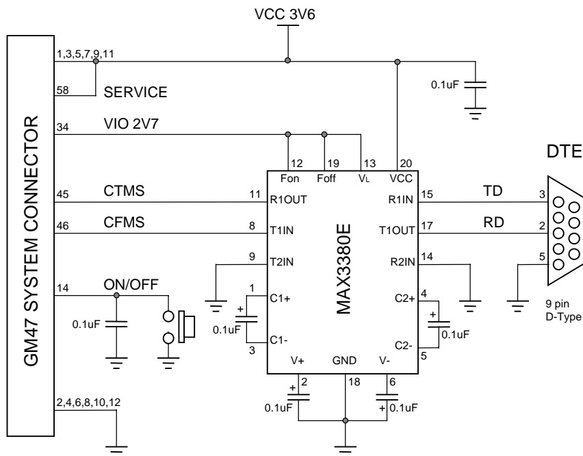
Figure 3.5 Service Circuitry
