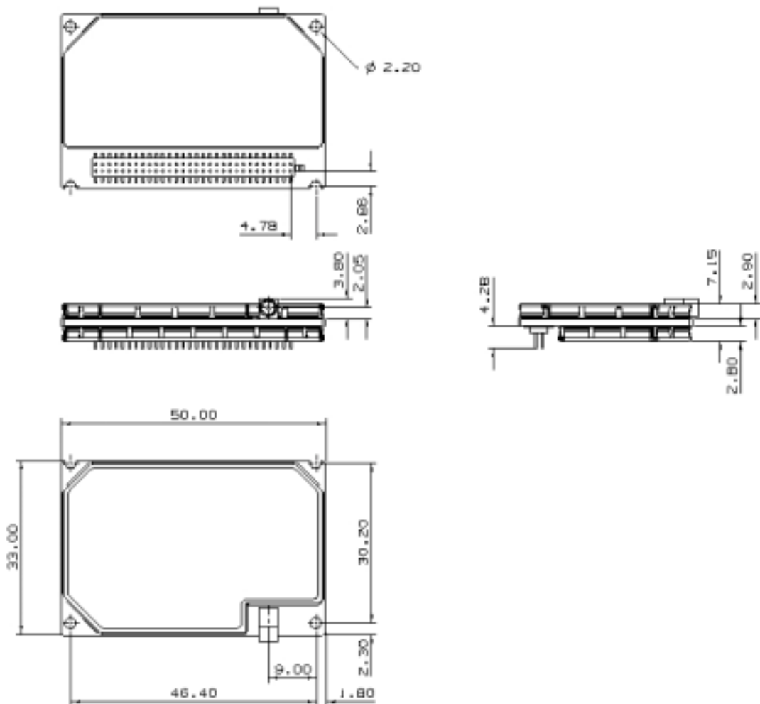
Figure 2.1 Physical dimensions of GM 47/48
